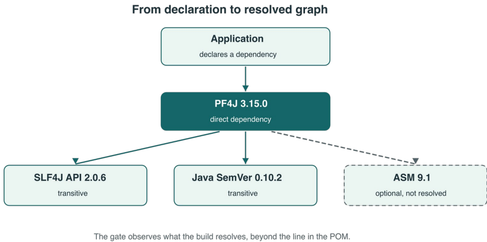
Figure 9.1 — The project declares PF4J; Maven resolves two transitive components. ASM is declared optional by the producer and does not enter the observed runtime tree.
