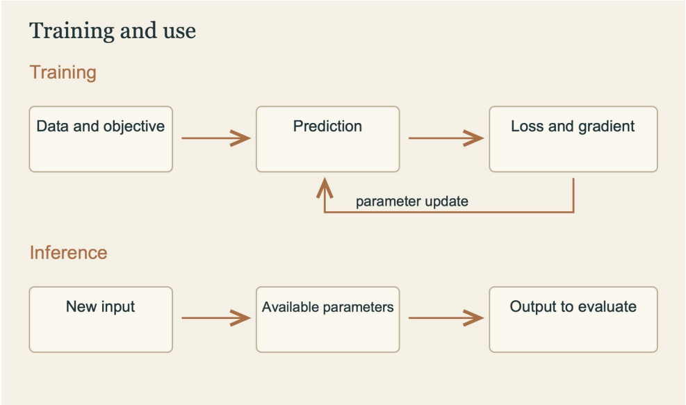
Figure 2 · Training and using a network are different processes
