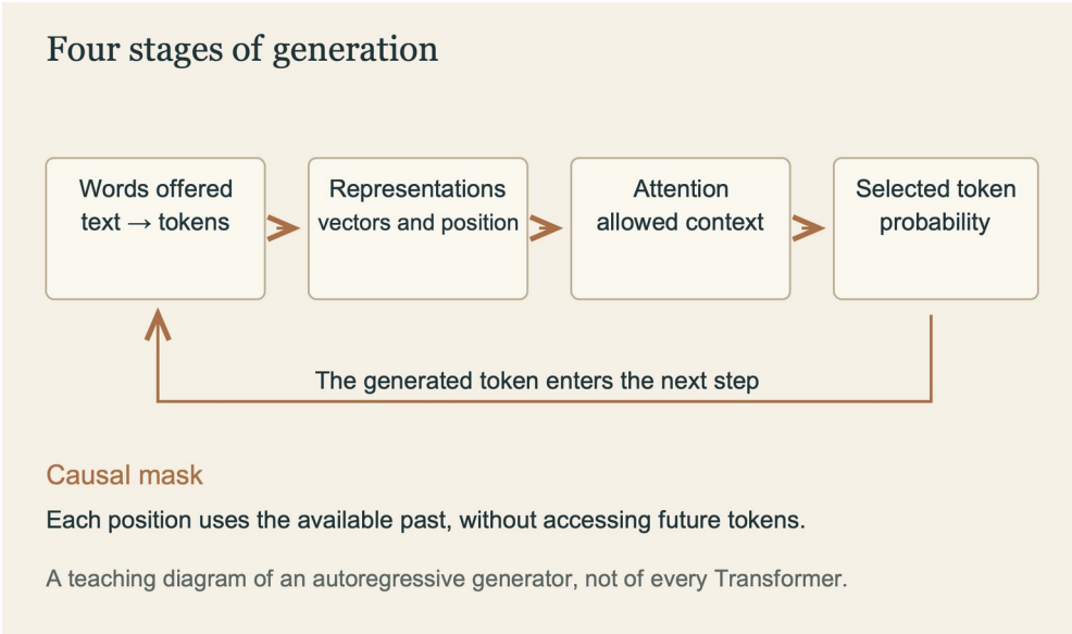
Figure 3 · Four stages of generation
